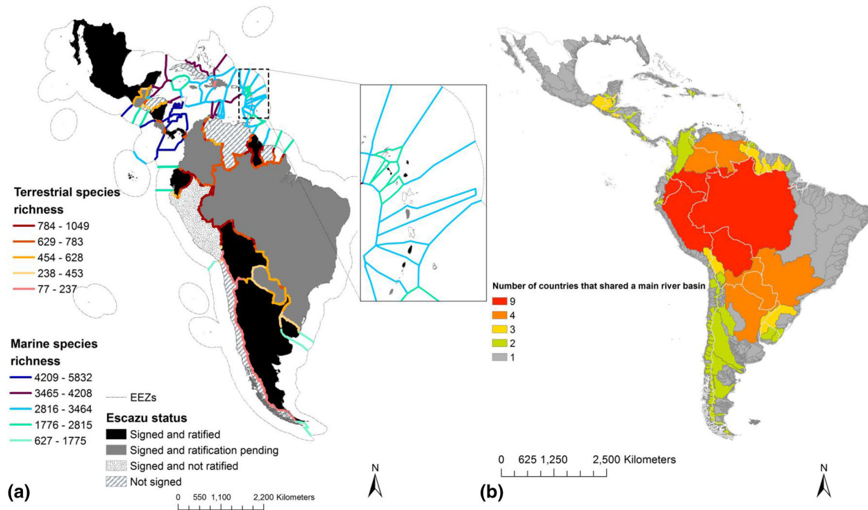
FIGURE 2 Terrestrial (mammals, birds, and amphibians, red gradient) and marine (marine and semimarine animals, except amphibians, blue gradient) species richness with transboundary ranges across each border and Escazú status. (b) River basins according to the number of countries they span. Abbreviation: EEZ, exclusive economic zone
